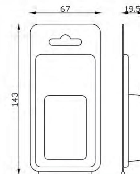
Blister Q (for Plastic box 6)
