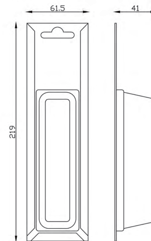
Blister 5 (with foam bed)
