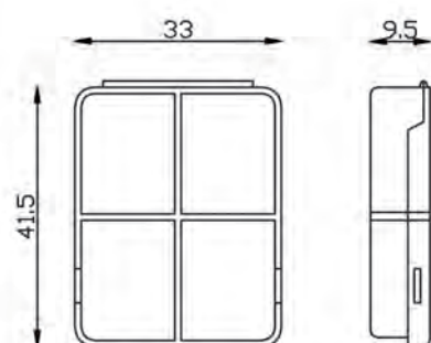
Plastic box 2 (fits perfectly in Blister B)
