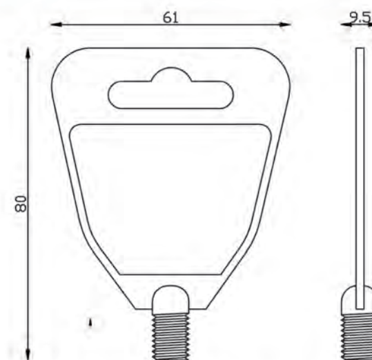
Bankstick & buzzerbar hangtag
