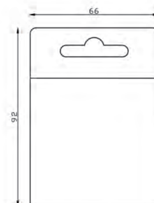
PET blisterbox (for Spool 4)
