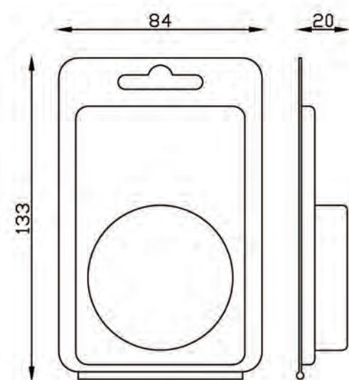
Blister X (for Spool 3)
