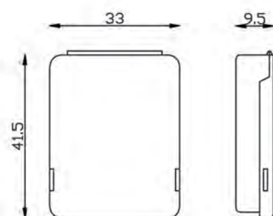
Plastic box 1 (fits perfectly in Blister B)
