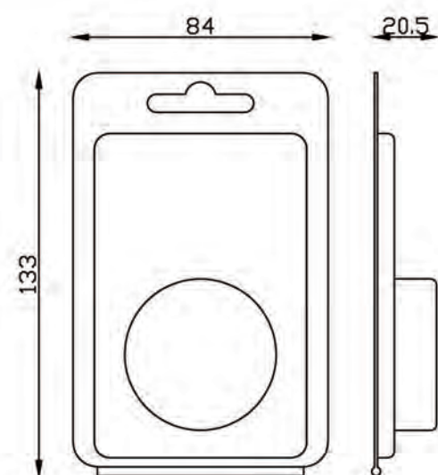
Blister W (for Spool 2)
