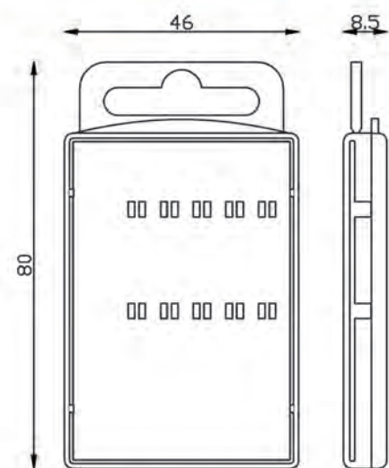
Special hook box 1
