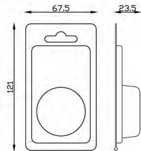
Blister S (for Spool 1)
